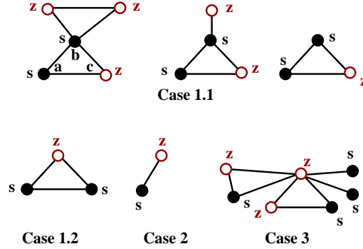
Figure 4: The cases
