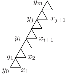
Figure 1: Path
