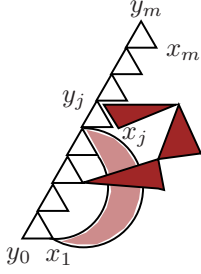
Figure 2: Ladder
