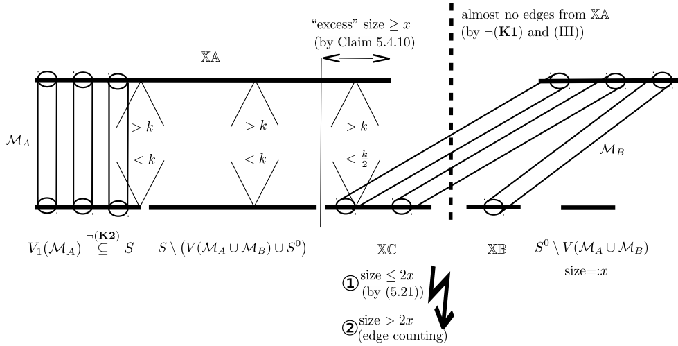
FIG. 5. A simplified computation showing that \neg(\mathbf{K1}) and \neg(\mathbf{K2}) lead to a contradiction. Denoting by x the size of S^0 \setminus V(\mathcal{M}_A \cup \mathcal{M}_B) , we get ① |\mathbb{X}\mathbb{C}| \leq 2x . On the other hand, each vertex of \mathbb{X}\mathbb{A} emanates \gtrsim k edges which are absorbed by the sets V_1(\mathcal{M}_A) , S \setminus (V(\mathcal{M}_A \cup \mathcal{M}_B) \cup S^0) , and \mathbb{X}\mathbb{C} . The vertices of V_1(\mathcal{M}_A) and S \setminus (V(\mathcal{M}_A \cup \mathcal{M}_B) \cup S^0) can absorb \lesssim k edges. The vertices of \mathbb{X}\mathbb{C} receive \lesssim \frac{k}{2} edges of \mathbb{X}\mathbb{A} by (5.24). This leads to ② |\mathbb{X}\mathbb{C}| > 2x , doubling the size of the “excess” vertices of \mathbb{X}\mathbb{A} .
