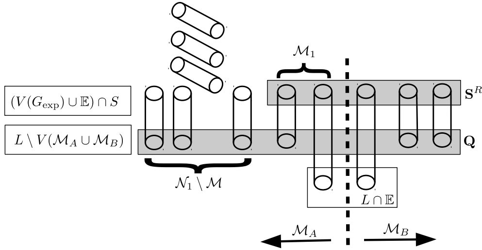
FIG. 4. The situation in G after applying Lemma 4.8. The dotted line illustrates the separation as in (III).
