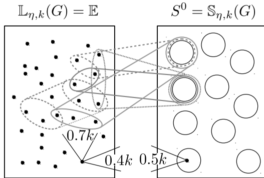
FIG. 3. An example of a graph G \in \mathbf{LKS}(n, k, \eta := \frac{1}{10}) in which \mathbf{G}_{\text{reg}} is empty, yet there is no candidate set for \mathbb{X}\mathbb{A} of vertices which have degrees at least k outside the set S^0 . Sample dense spots are shown in gray.
