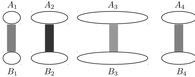
FIG. 1. An example of an (\varepsilon, d, \ell) -regularized matching. Regular pairs are shown with a shade of gray corresponding to their densities.
