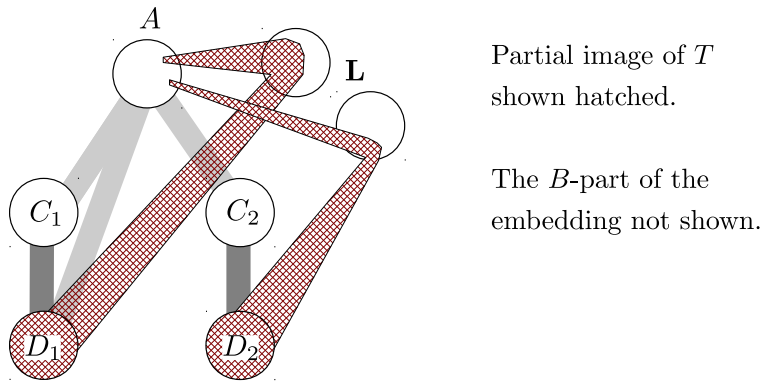
FIG. 2. The reason for requiring (5.2) in the setting of (H2). Consider two edges C_1D_1, C_2D_2 \in M such that only C_2D_2 satisfies (5.2). At some point during the embedding of T , we may need to use the high-degree property of clusters in \mathbf{L} . When doing so we cannot guarantee that we will fill the edges of M in an efficient way. That is, we may end up filling D_1 and D_2 completely and leaving C_1 and C_2 untouched. If this happens, both regular pairs C_1D_1 and C_2D_2 are useless for embedding further shrubs. The used space in C_2D_2 equals the degree from A to C_2D_2 . That is, we do not expect to embed anything more in the edge C_2D_2 . The condition \deg_{\mathbf{G}_{\text{reg}}}(A, \mathbf{L} \cup V(M)) \geq K ensures that we find free space somewhere else in the cluster graph to complete our embedding. Clearly, the pair C_1D_1 does not have this favorable feature: The number of vertices used by the embedding is only half the degree of A to C_1D_1 . In this case, the condition \deg_{\mathbf{G}_{\text{reg}}}(A, \mathbf{L} \cup V(M)) \geq K is not strong enough. We do not need a counterpart of (5.2) for \mathbf{N}_{\mathbf{G}_{\text{reg}}}(B) . The reason is that we can schedule our embedding process in such a way that when we use the high-degree property of \mathbf{L} we have already exhausted the degree from B to M .
